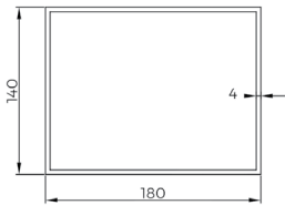
4 Column profile
