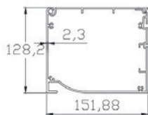
6 Motor Box Profile
