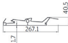
7 Lamella profile
