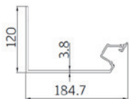
5 Side Gutter Profile
