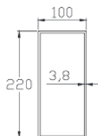
2 Column and Side Beam Profile
