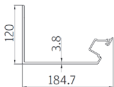
5 Side Gutter Profile
