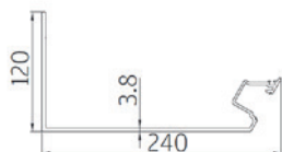
1 Front and Back Gutter Profile
