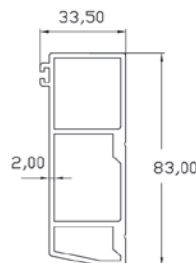
4 Front Profile
