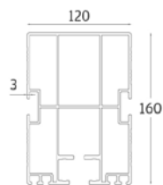
1 Rafter Profile
