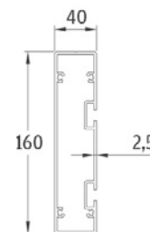
6 Motor Box Profile
