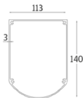
3 Column Profile
