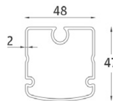
5 Fabric Profile | Carrier
