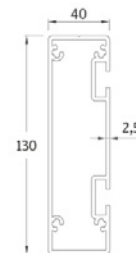
5 Fabric Profile | Carrier 6 Motor Box Profile
