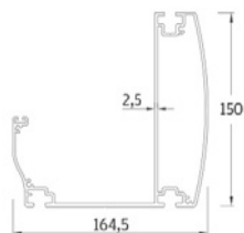
2 Gutter Profile
