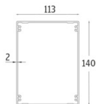
3 Column Profile
