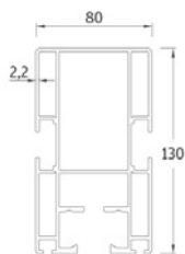
1 Rafter Profile
